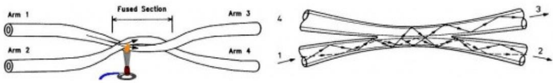
Figura 2.17 Fused Biconic Taper FBT
