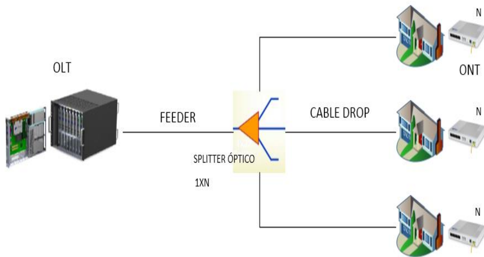
Figura 2.28 FTTH (Fiber to the Home)
